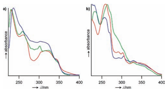
Figure 2. Absorption spectra in CH 2 Cl 2 (10 −5 M) of (a) phosphole-containing \pi -systems 6a (red), 6b (blue), and 6c (green), and (b) their corresponding oxides 7a (red), 7b (blue), and 7c (green).
