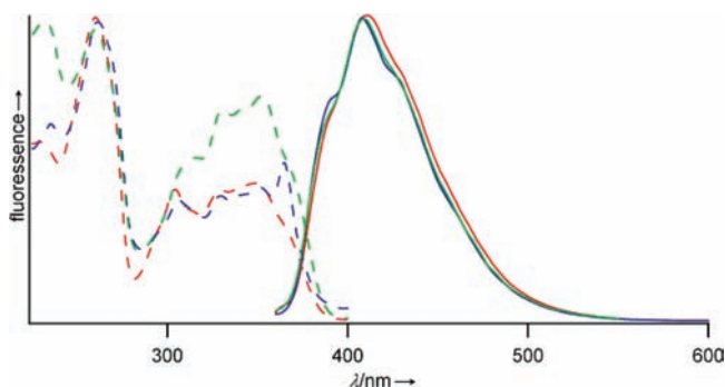
Figure 6. Fluorescence (solid) and excitation spectra (dotted) of phosphole-oxide-containing \pi -systems 7a (red), 7b (blue), and 7c (green) in cyclohexane ( 10^{-6} M; \lambda_{\text{exc}} = 350 nm; \lambda_{\text{em}} = 410 nm).
